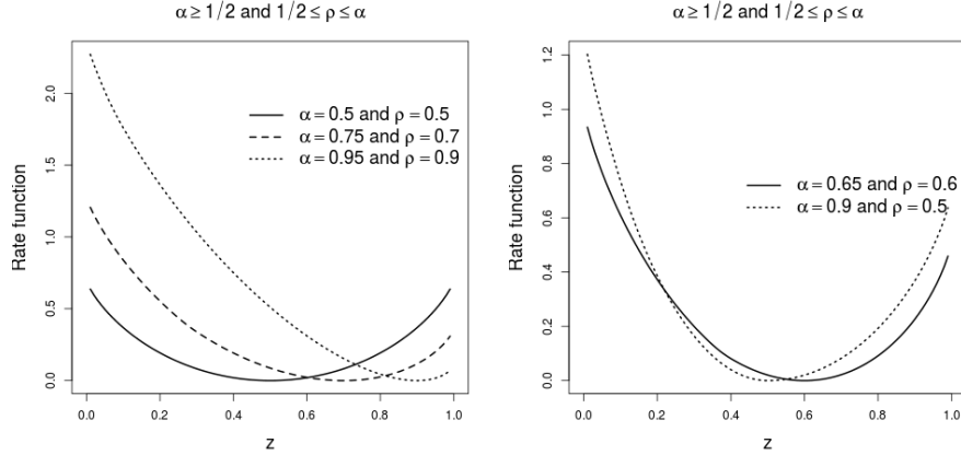
FIGURE 2. Rate functions for case (c) of Theorem 2.2.
