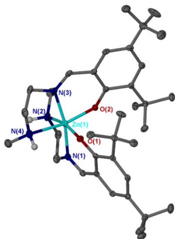
Figure 1. Solid-state structure of Zn(1). Ellipsoids shown at 30 % probability level and all hydrogen atoms, except those bound to nitrogen have been omitted for clarity.
