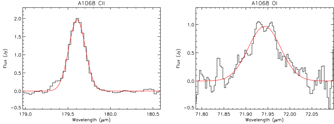
Fig. 1. Herschel PACS spectra of [CII] and [OI] in A1068
