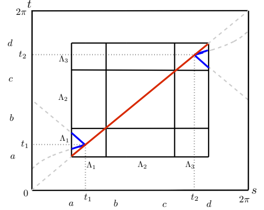
Figure 4.12: The boundaries of the illuminated \Lambda_2 := [b, c] and transition domains \Lambda_1 := [a, b] and \Lambda_3 := [c, d] are plotted along with the diagonal s = t in red and blue curves representing points where Hypothesis A is not satisfied within the domain contained in the rectangles.
