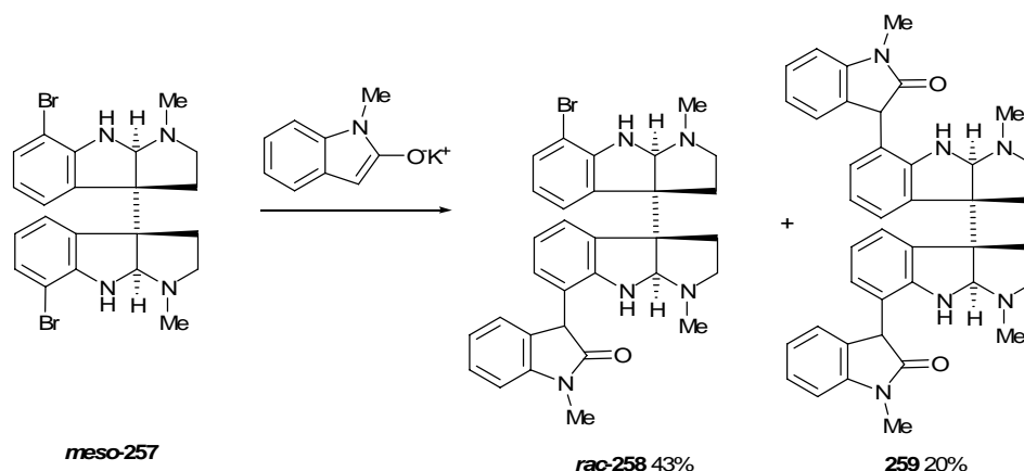
Scheme 6.2: Reagents and Conditions: oxindole 22 (1.0 equiv.), bisamine meso-257 (2.0 equiv), NaH (4.05 eq.), Pd(dba) 2 (2 mol%), X-Phos L30 (3 mol%), KHMDS (1.1 equiv), THF, 70 °C.
