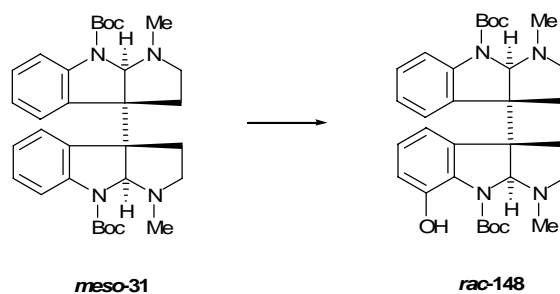
Scheme 4.10: Reagents and Conditions: biscarbamate meso - 31 (1 eq.), sec -BuLi (4.5 eq.), TMEDA (6 eq.), THF, -78\text{ }^\circ\text{C} , then (\text{TMSO})_2 139 (5 eq.), THF, -78\text{ }^\circ\text{C} to r.t.
