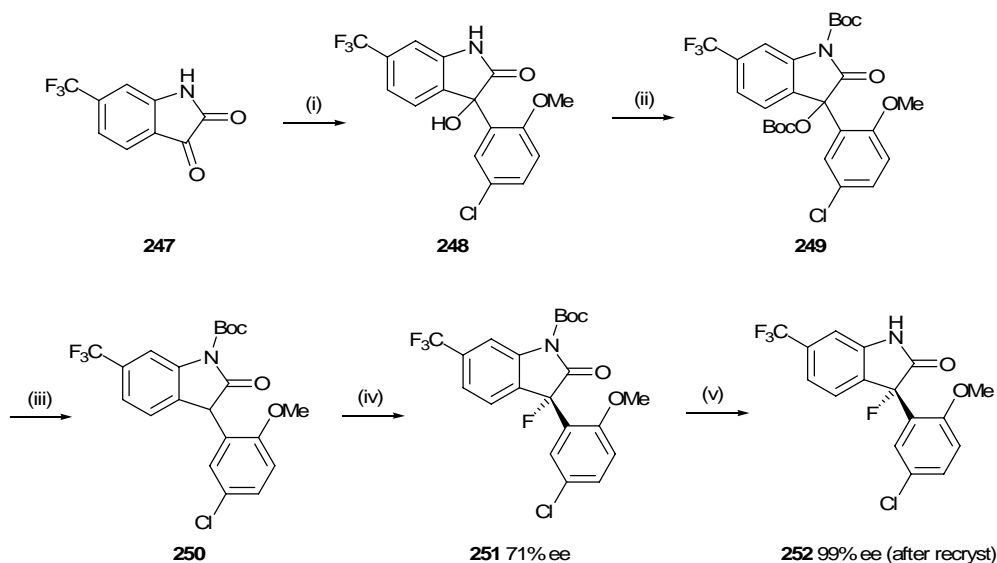
Scheme 5.7: Reagents and Conditions: (i) isatin 247 (1 eq.), aryl-MgBr (2 eq.), THF, -40 °C; (ii) (Boc) 2 O (2 eq.), DMAP (0.1 eq.), DCM; (iii) Pd(OH) 2 , H 2 , MeOH-EtOAc; (iv) [PdOH((S)-DM-BINAP) (S)-L3] 2 (2.5 mol%), NFSI (1.5 eq.), acetone, 0 °C; (v) TFA, DCM.
