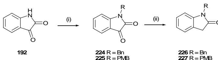
Scheme 5.4: Reagents and Conditions: (i) isatin (1 eq.), NaH (1.05 eq.), 0 °C, DMF, 30 min then alkyl bromide (1.2 eq.), 45 min; (ii) N 2 H 4 .H 2 O neat, reflux.
