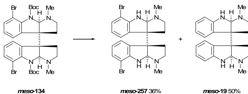
Scheme 6.1: Reagents and Conditions: TMS-OTf (4.4 eq.), DCM, 8 h, r.t.
