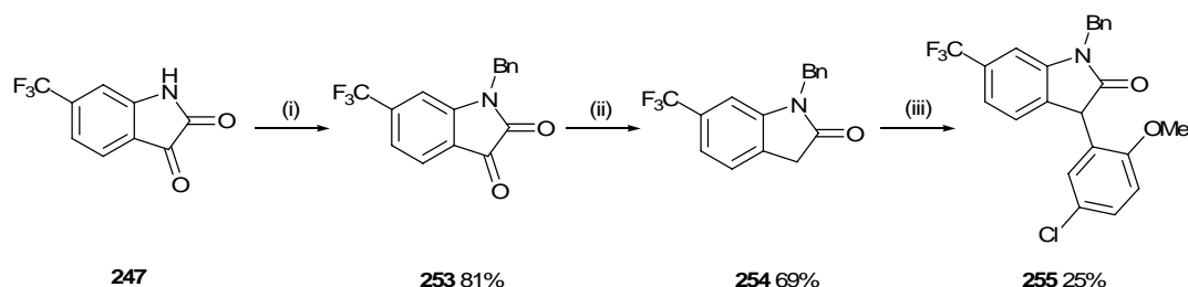
Scheme 5.8: Reagents and Conditions: (i) isatin 247 (1 eq.), NaH (1.05 eq.), 0 °C, DMF, 30 min then BnBr (1.2 eq.), 45 min; (ii) N 2 H 4 ·H 2 O neat, reflux; (iii) arene (1.1 equiv), Pd(dba) 2 (2 mol%), X-Phos L30 (3 mol%), KHMDS (1.1 equiv), THF, 70 °C, 30 mins.
