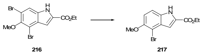
Scheme 5.1: Reagents and Conditions: dibromide 216 (1 eq.), Pd(OAc) 2 , (5 mol%), rac -BINAP rac - L1 (5.5 mol%), TMEDA (1.5 eq.), NaBH 4 (1 eq., 0.5 M in diglyme), THF, 50 °C, 24 h.
