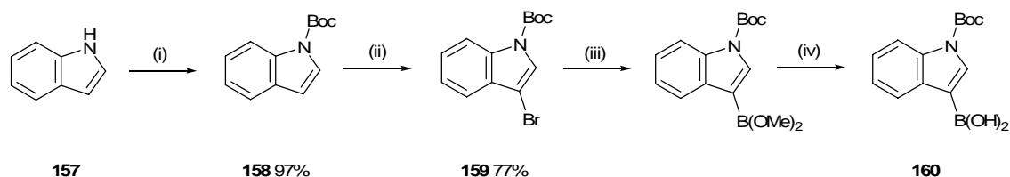
Scheme 4.20: Reagents and Conditions: indole 157 (1 eq.), (Boc) 2 O (1.1 eq.), DMAP (0.01 eq.), THF; (ii) NBS (1.3 eq.), THF; (iii) tert -BuLi (1.05 eq.), THF, -100 °C, 10 min. then B(OMe) 3 (2 eq.), -100 °C to r.t.; (iv) 3 M HCl.
