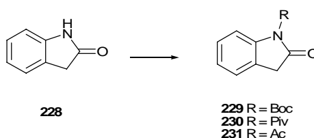
Scheme 5.5: Reagents and Conditions: oxindole 228 (1 eq.), anhydride (2.5 eq.), DMAP (cat.), Na 2 CO 3 , THF, 70 °C, reflux.
