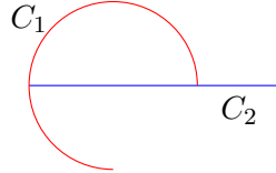
Example 2.10: subadjacency and closure finiteness II
