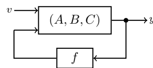
Figure 1.1: Lur'e system with linear part (A, B, C) , nonlinearity f , output y and input v
