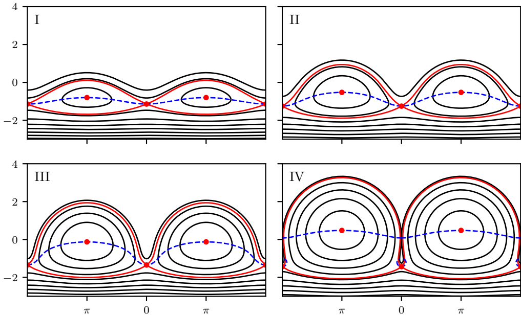
FIGURE 2. Free surfaces and streamlines, in the (x, y) plane, for the new exact solutions in (4.5) for A = A_{\max}/4 , A_{\max}/2 , 3A_{\max}/4 , and A_{\max} . Up to a vertical shift, the free surfaces I–IV coincide with the streamlines I–IV for the Crapper wave in Figure 1. The stagnation points are shown in red, together with the heteroclinic connections between the saddle points. These heteroclinic orbits enclose a so-called critical layer of closed streamlines, which in particular contains the dashed blue curve across which the horizontal velocity changes sign.
