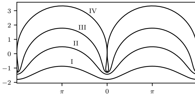
FIGURE 1. Streamlines for the limiting Crapper wave. Curve IV is the free surface. Alternatively, after an appropriate vertical shift, Curves I, II, III may be thought of as the free surface for the Crapper wave for different values of A and \tau .
