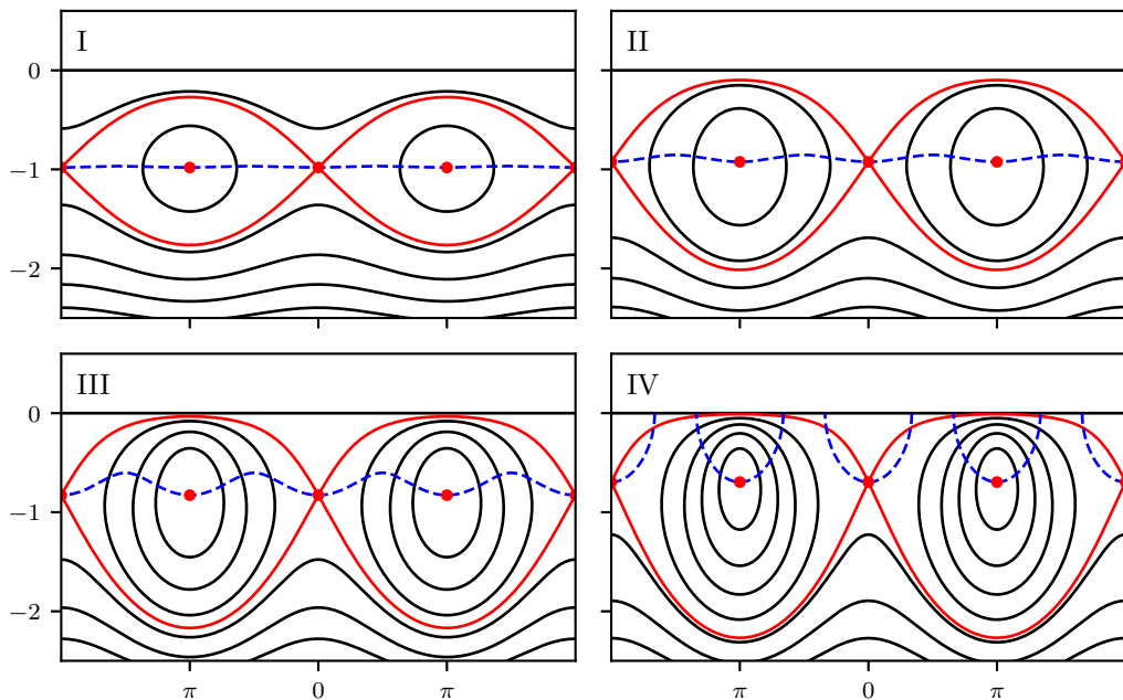
FIGURE 3. The examples from Figure 2 in the (\alpha, \beta) plane. Here the streamline \beta = 0 corresponds to the free surface. Note that the stagnation points in a given wave all have the same value of \beta .
