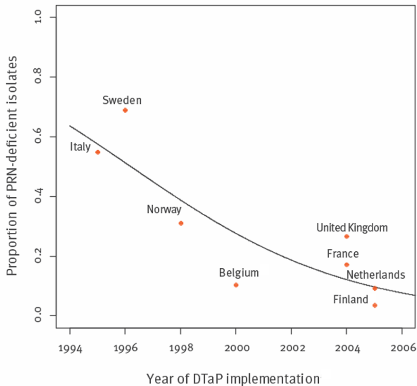
Figure 2: Correlation between the introduction of a primary acellular pertussis vaccine containing pertactin (PRN) in a European country and the proportion of PRN-deficient isolates found in the study, 2012–2015. Reproduced with permission from Barkoff et al. (2019)
