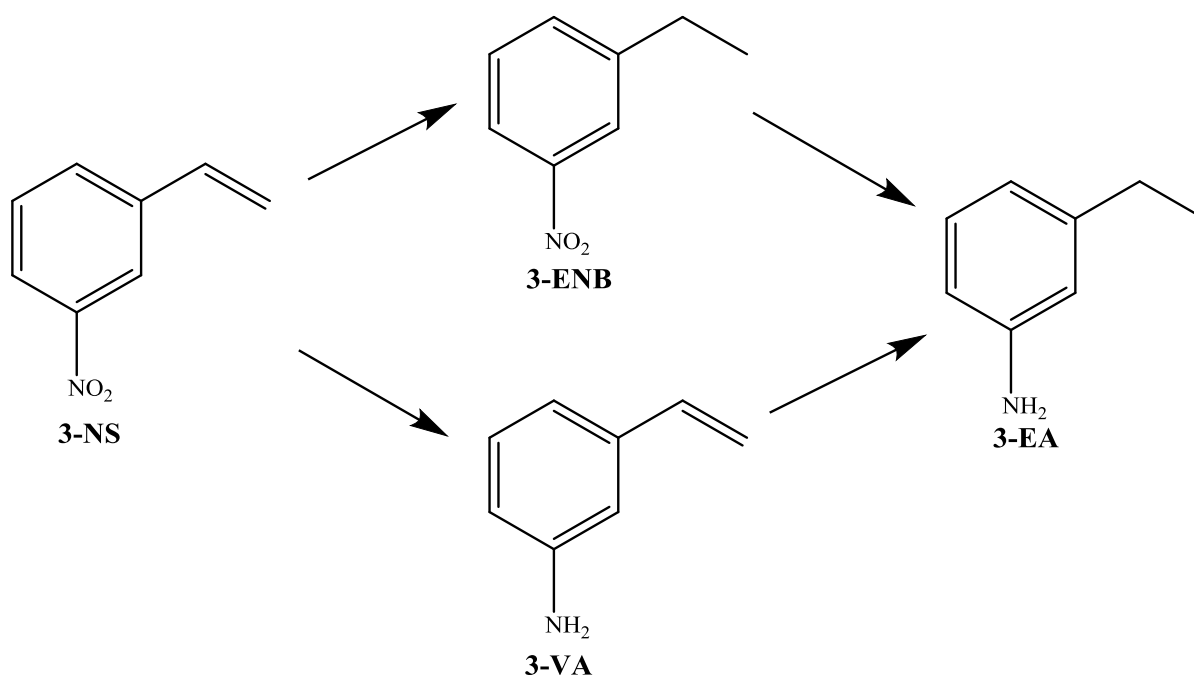
Scheme-1: Schematic representation of the chemoselective hydrogenation of 3-nitrostyrene (3-NS) to form the desired product 3-vinyylaniline (3-VA) and associated side products 3-ethylnitrobenzene (3-ENB), and 3-ethylaniline (3-EA).
