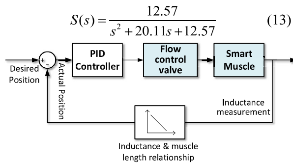
Figure 9: PID controller for smart muscles
