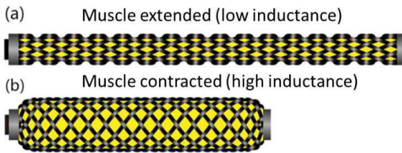
Figure 1: Smart sensing braid for measuring the deformation of a PAM
