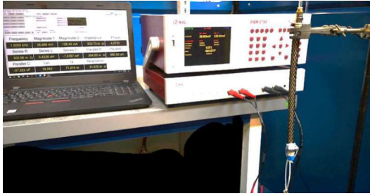
Figure 5: Inductance measurement using Newtons4thPSM3750 Phase Sensitive Multimeter
