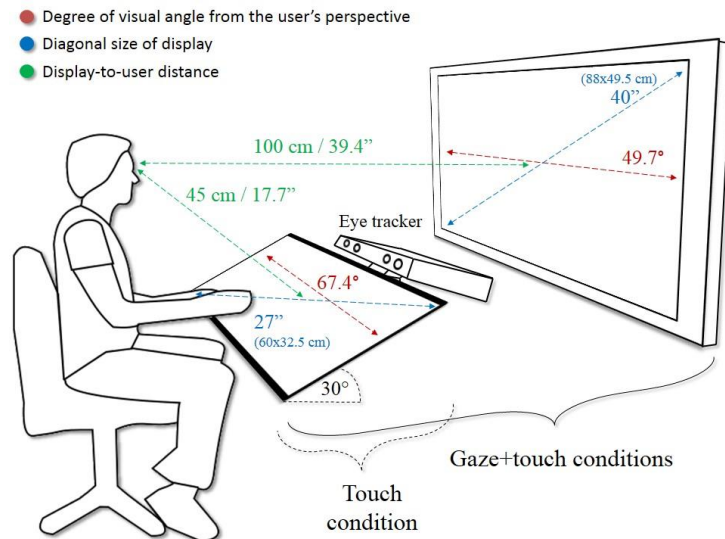
Fig. 2. Study setup.
