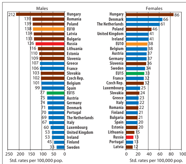
Figure 2. Lung cancer mortality in European Union countries and Russia, males and females, age group 45-64, 2008 (2006: Belgium, Denmark); blue and green – countries of Western Europe, brown, orange and red – countries of Central and Eastern Europe, including Russia. Source [1]
