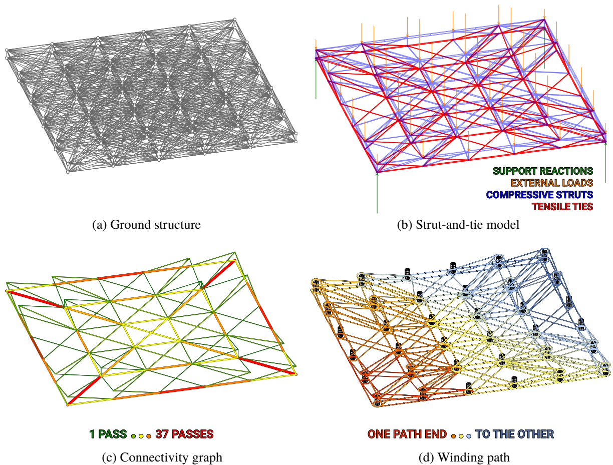
Figure 8. Automated optimisation and rationalisation of a reinforcement layout suitable for robotic filament winding for a concrete plate.
