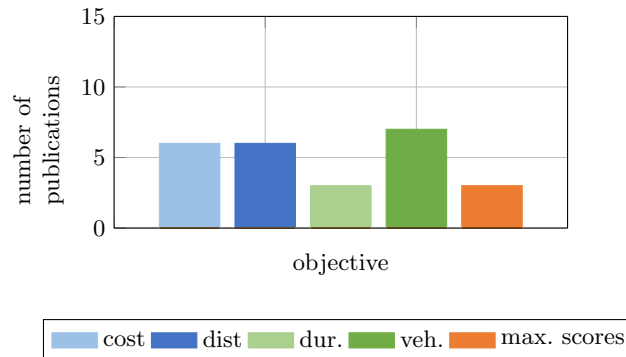
Figure 11 Objectives for intermediate stops for break and rest periods.
