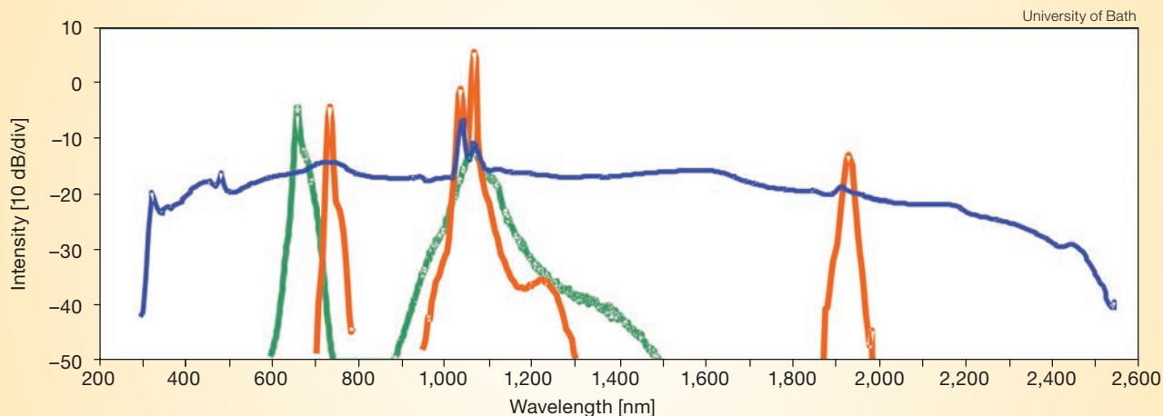
Comparison of a supercontinuum (blue line) with four-wave mixing (FWM) (orange and green lines). The continuum spans the entire UV-visible-NIR with a smooth spectrum and a relatively low spectral power density. FWM in two different photonic crystal fibers generates high-power density at specific wavelengths for applications such as STED microscopy.
