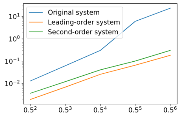
(b) Average runtime in seconds to solve (6), (9) and (50) for different values of \epsilon .
