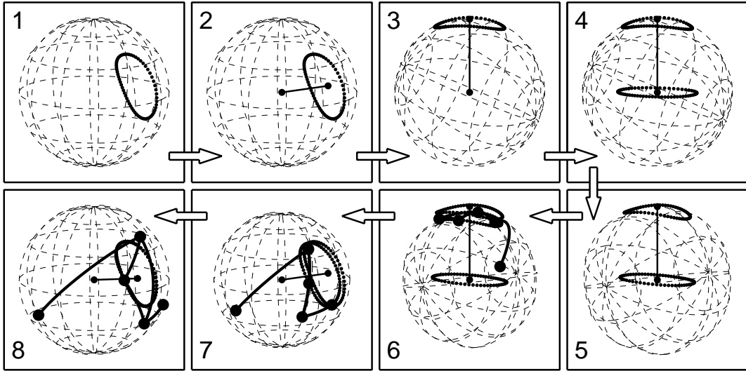
Figure 4: Normalizing a curve and unnormalizing a mechanism
