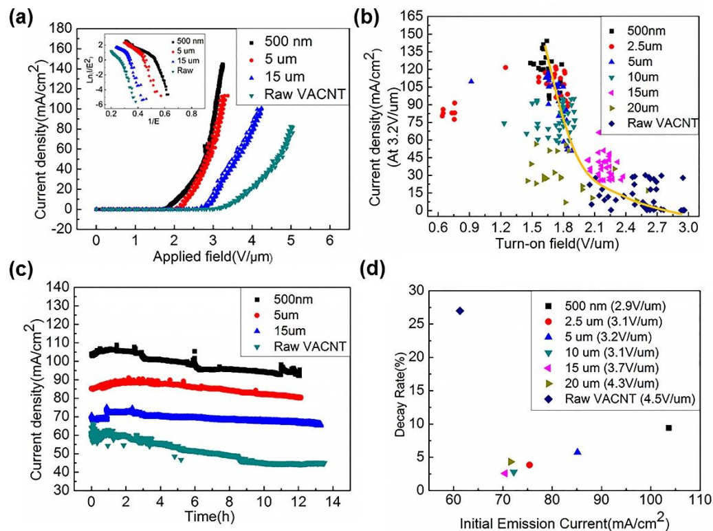
Figure 4. (a) Current density-Applied field curves of the raw VACNT film, the cone arrays of the tip size are about 500 nm, 5 \mu\text{m} , 15 \mu\text{m} , the illustration is Fowler-Nordheim plots. (b) The statistical diagram of the relationship between the open field strength and the current density of the unprocessed samples and the cone array samples with different tip sizes. (c) Current-Time stability curves of the raw VACNT film, the cone arrays of the tip size are 500 nm, 5 \mu\text{m} , 15 \mu\text{m} . (d) The relationship between the current decay rate (12 hours) and the initial current of raw samples and cone array samples with different tip sizes was studied. (The calculated emission is 4 \text{mm}^2 from Figure 4(a)-(d) ).
