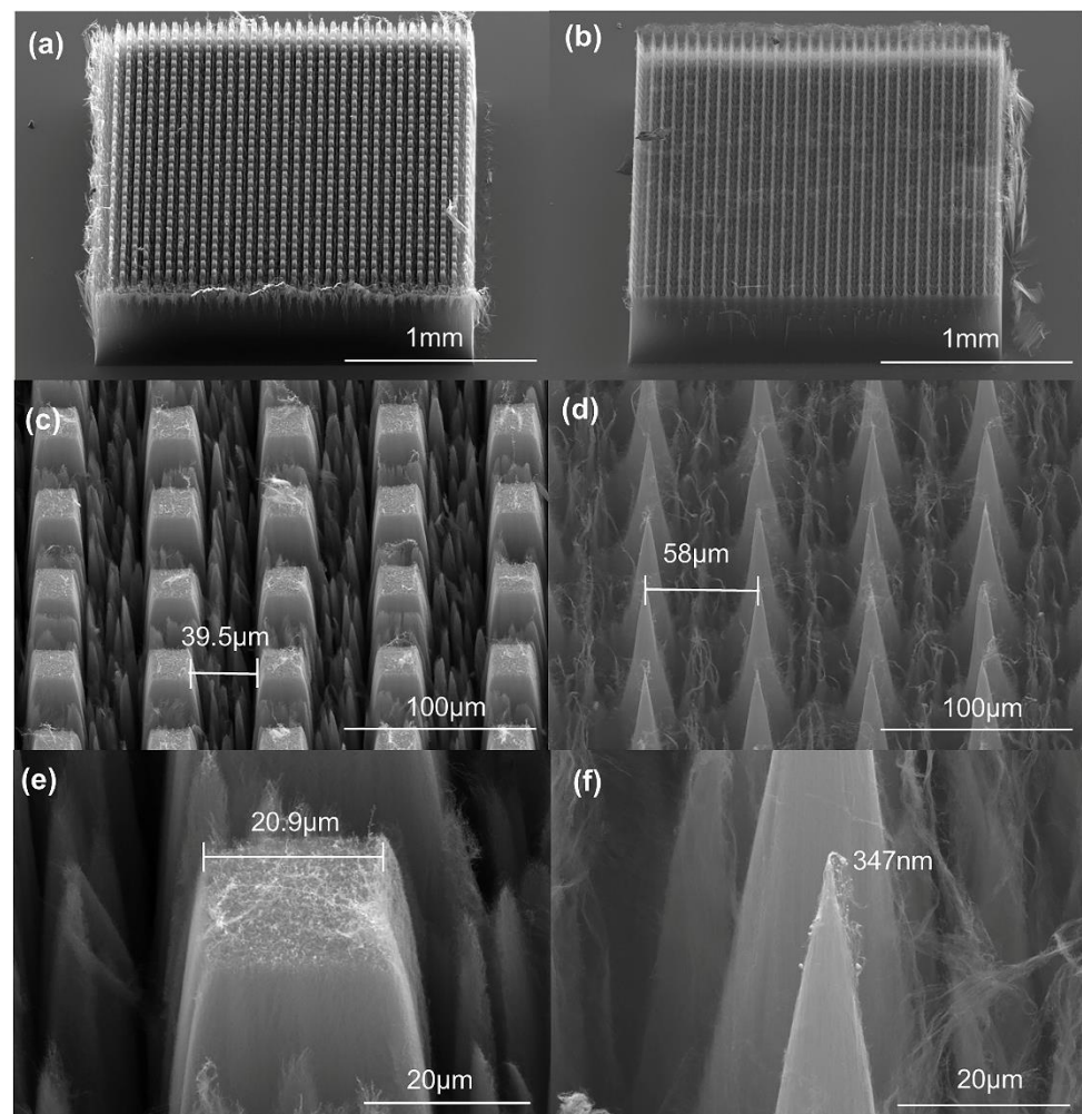
Figure 3. (a) A typical UV laser processed cuboid array with a side length of about 20 \mu\text{m} and (b) 500 nm consisting of 1089 elements. (c) An enlarged view of the processed array showing the formed tips about 20 \mu\text{m} and (d) about 500 nm. (e) A single tip in the array with a radius of curvature of 20.9 \mu\text{m} and (f) 347 nm.
