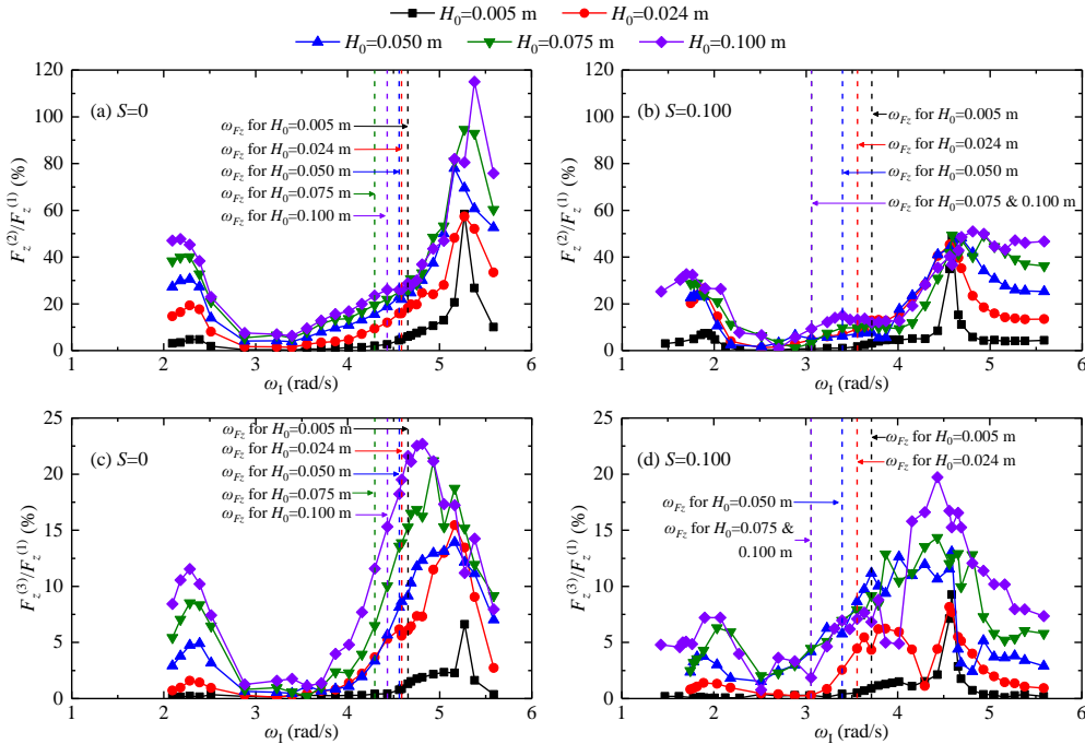
Fig. 7. Ratios of the high-order to the 1 st -order vertical wave forces under conditions of S=0 and 0.100. (a) and (b) correspond to the ratios of the 2 nd - to the 1 st -order ones, and (c) and (d) correspond to the ratios of the 3 rd - to the 1 st -order ones. F_z^{(m)} ( m=1, 2 and 3) denote the m^{\text{th}} -order vertical wave force.
