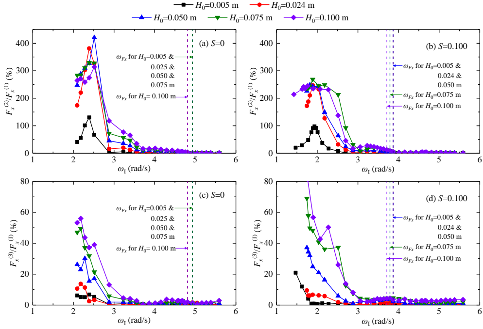
Fig. 10. Ratios of the high-order to the 1 st -order horizontal wave forces under conditions of S=0 and 0.100. (a)-(b) correspond to the ratios of the 2 nd - to the 1 st -order ones, and (c)-(d) correspond to the ratios of the 3 rd - to the 1 st -order ones. F_x^{(m)} ( m=1, 2 and 3) denote the m^{\text{th}} -order horizontal wave force.
