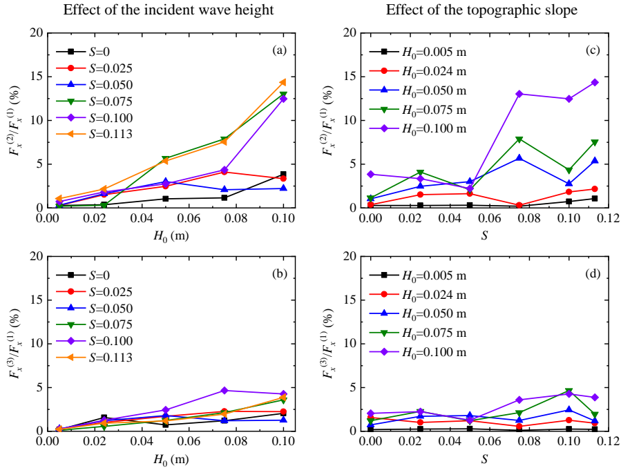
Fig. 11. Variations of both F_x^{(2)}/F_x^{(1)} and F_x^{(3)}/F_x^{(1)} at \omega_{Fx} with respect to the incident wave height H_0 (a and b) and to the topographic slope S (c and d).
