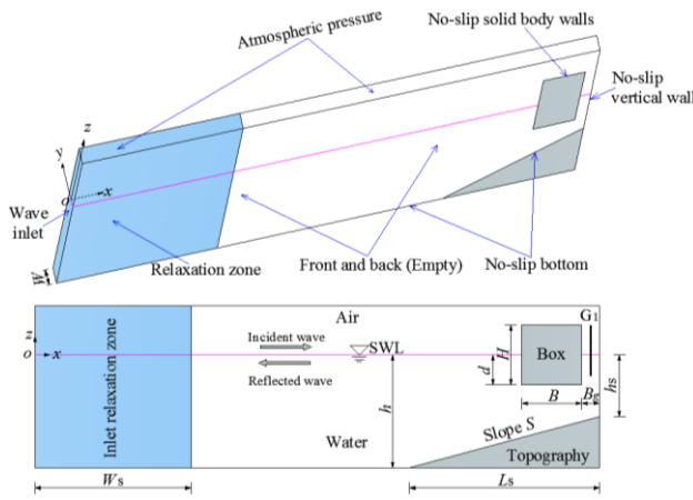
Fig. 1. Definition sketch of the numerical wave tank (NWT): the boundary conditions and the
