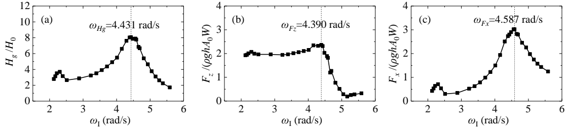
Fig. 2. Variations of (a) the total wave height in the gap, (b) the total vertical wave force, and (c) the total horizontal wave force with respect to the incident wave frequency, \omega_1 , for H_0=0.024 m and S=0.050 .
