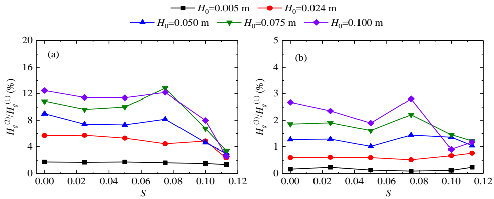
Fig. 6. Variations of (a) H_g^{(2)}/H_g^{(1)} and (b) H_g^{(3)}/H_g^{(1)} at the fluid resonant frequency with respect to
