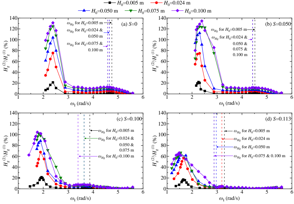
Fig. 3. Ratios of the 2 nd - to the 1 st -order wave heights inside the gap for all cases under conditions of S=0, 0.050, 0.100, and 0.113 . H_g^{(1)} and H_g^{(2)} denote the 1 st and the 2 nd -order wave heights in the gap, respectively.
