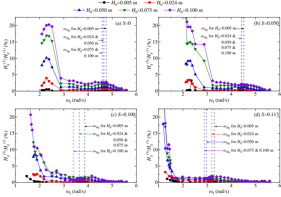
Fig. 4. Ratios of the 3 rd - to the 1 st -order wave heights inside the gap for all cases, in which H_g^{(3)} denotes the 3 rd -order wave heights in the gap.
