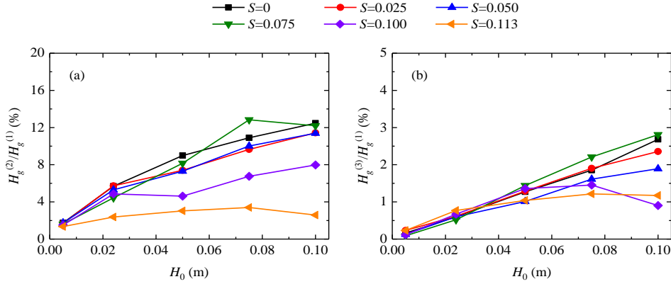
Fig. 5. Variations of (a) H_g^{(2)}/H_g^{(1)} and (b) H_g^{(3)}/H_g^{(1)} at the fluid resonant frequency with respect to the incident wave height, H_0 , for all the topographic slopes.
