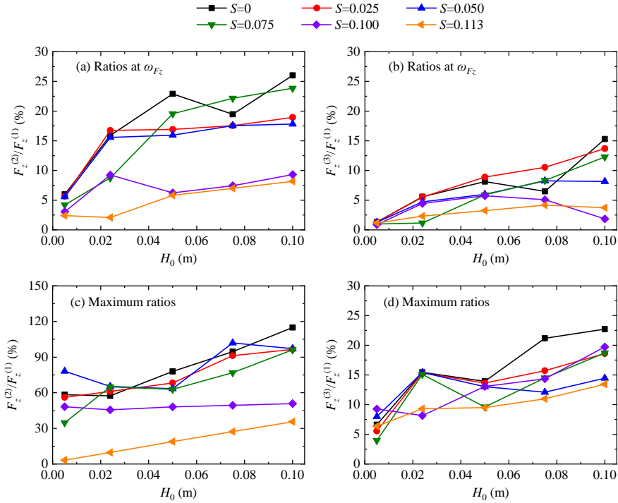
Fig. 8. Variations of the ratios of the high-order vertical wave forces at \omega_{F_z} and their maximum ratios with respect to H_0 for all the topographic slopes. (a) and (b) correspond to F_z^{(2)}/F_z^{(1)} and
