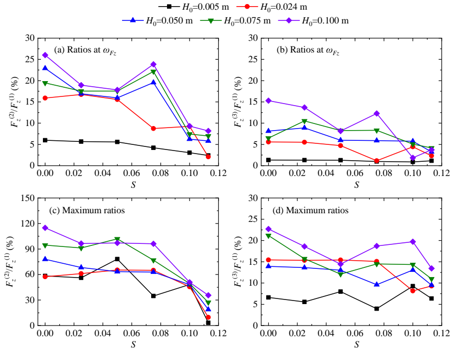
Fig. 9. As in Fig. 8, but for the variations of the ratios of the high-order vertical wave forces with respect to S for all the incident wave heights.
