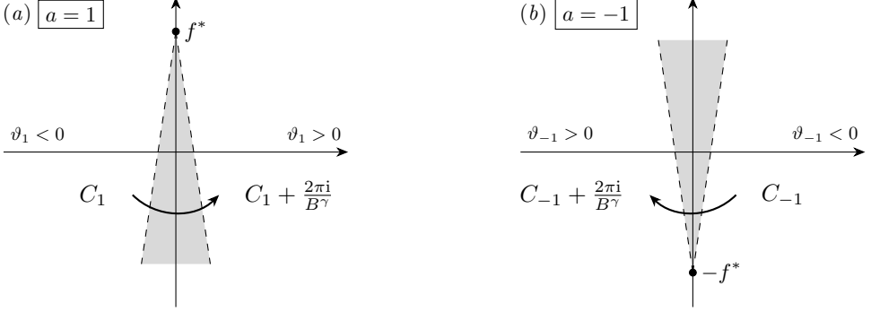
Figure 8: The Stokes smoothing procedure is visualised for a = 1 in (a) and for a = -1 in (b).
