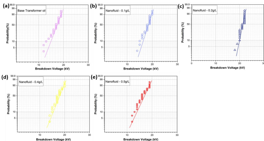
Figure.5. Weibull distribution of the AC breakdown voltage of the transformer oil and nanofluid for a different concentration of ZrO 2 nanoparticles.
