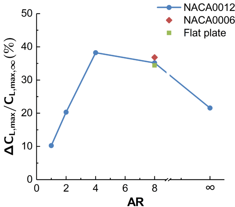
Figure 7: Percentage increase of maximum lift coefficient as a function of aspect ratio.
