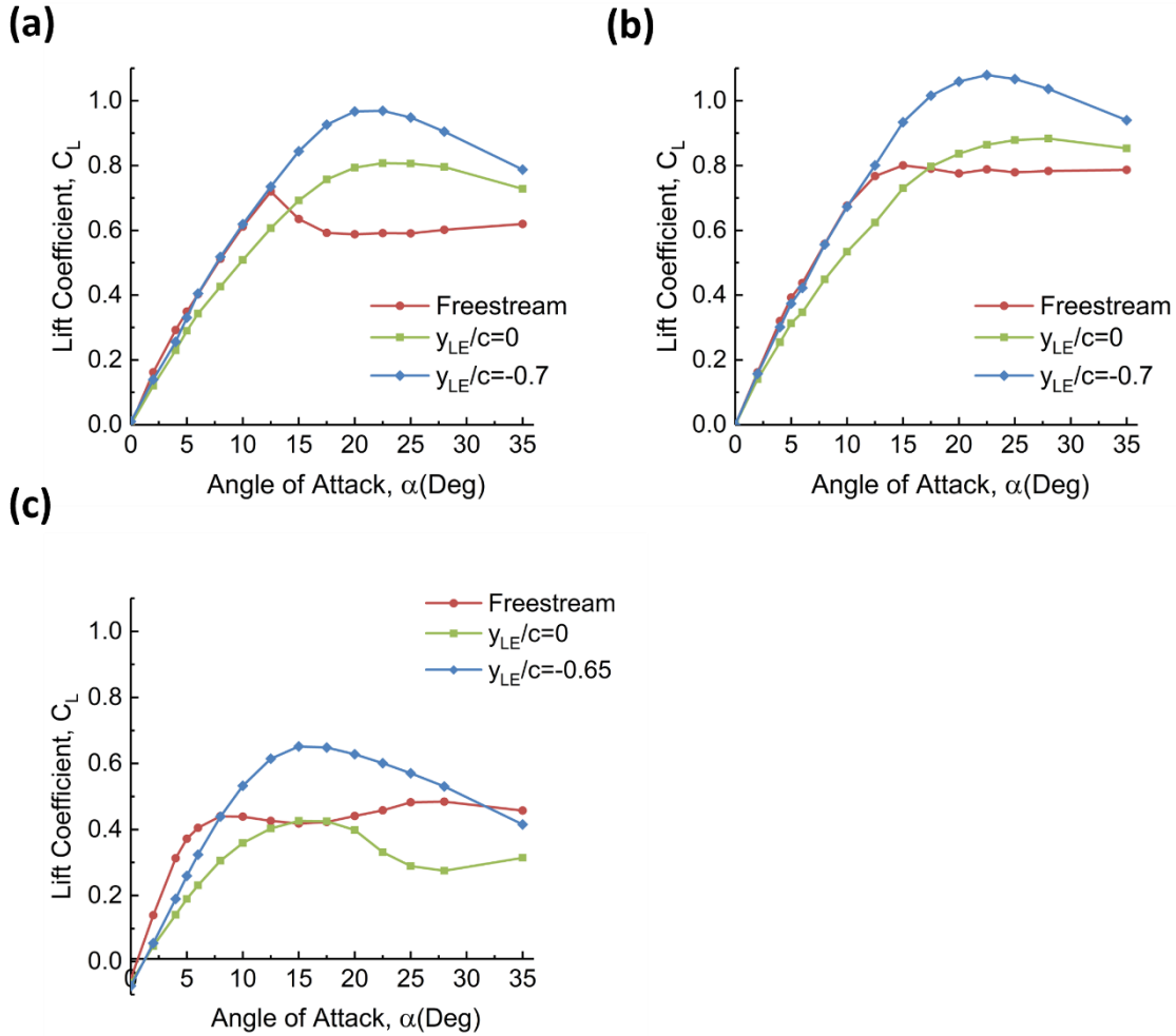
Figure 15: Time-averaged lift coefficient as a function of angle of attack for (a) NACA0012; (b) NACA0006; (c) flat plate; AR=8 .
