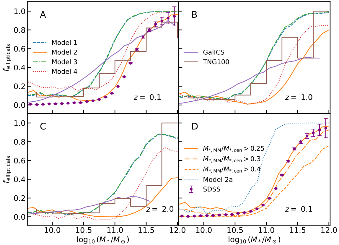
Figure 10. Fraction of elliptical galaxies as a function of the galaxy stellar mass as predicted by DECODE. Panels A, B and C show the predictions for the four models described in Section 4.1 at redshifts z = 0.1 , 1 and 2, respectively. Panel D shows the predictions for Model 2 at redshift z = 0.1 , along with the impact of assuming different mass ratio for the major mergers (denoted as MM in the legend), as well as the prediction for Model 2a. The data from the SDSS Survey, GALICS semi-analytic model and the TNG100 hydrodynamical simulation are included, as labelled, for comparison.
