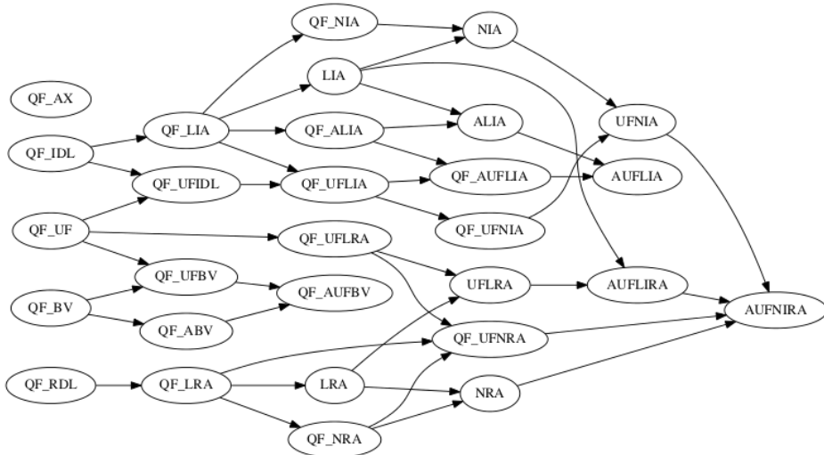
Figure 1.2. Available logics (March 2022) https://smtlib.cs.uiowa.edu/logics.shtml
