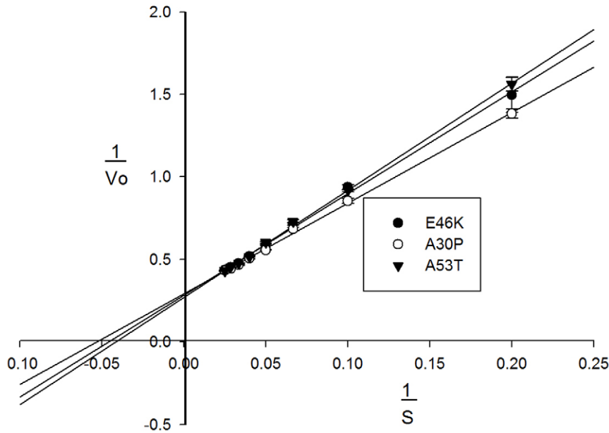
Figure 3. Comparison of the ferrireductase activity of the disease associated \alpha S mutants. doi:10.1371/journal.pone.0015814.g003
