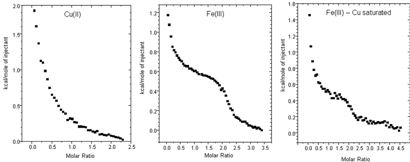
Figure 1. ITC analysis of copper and iron binding. ITC traces for titrations of Cu (II) or Fe (III) into 100 \mu\text{M} \alpha\text{S} at pH 7, 25°C. An isotherm for the titration of Fe (III) into Cu (II) loaded protein is also shown (far right). doi:10.1371/journal.pone.0015814.g001
