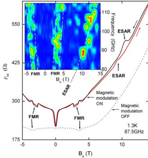
FIGURE 1. Magnetoconductance of a GaAs/AlGaAs 2DEG modulated by a sinusoidal magnetic field of amplitude 0.14T and period 400nm. The current is parallel to magnetic field domains. B_a is applied in the plane of the 2DEG either perpendicular to the cobalt stripes (magnetic modulation ON) or parallel to them (modulation OFF). Inset: frequency dependence of the ferromagnetic resonance (FMR) and electron spin anti-resonance (ESAR). The slopes are inversely proportional to the Landé g -factor in the metal ( g=2 ) and the GaAs quantum well ( g^*=0.42 ).
