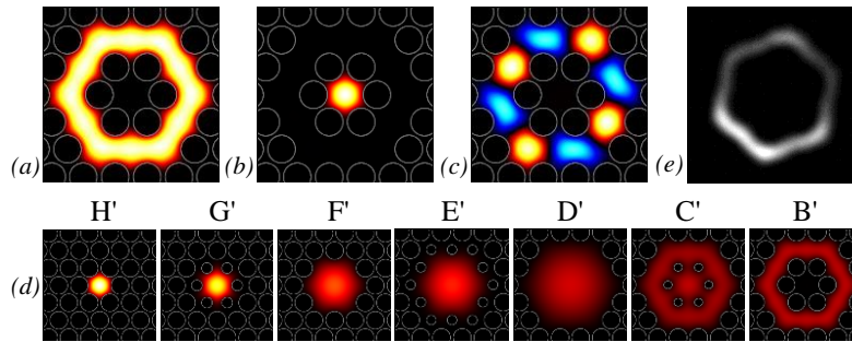
Fig. 7. (a)–(c) Calculated fields at B, for (a) the fundamental mode, (b) the 10th mode and (c) the 9th mode. (d) Simulated fields at locations H'–B' along a reverse mode convertor, for an LP 01 input at H' (Media 2). An LP 02 input at H' would give the reverse of Fig. 6(a). (e) Experimental near-field pattern at the end of a reverse transition H'–B', for input light of wavelength 800 nm in the LP 01 mode at H'.
