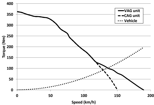
Fig. 15. Minimum driving torque for Transit and maximum torque profiles for VAG and CAG motors
