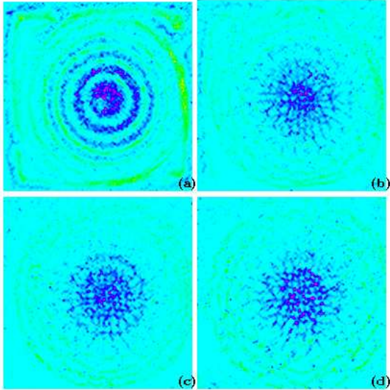
FIG. 3. (a) - (d) Vorticity maps ( \omega = \nabla \times \mathbf{u} ) highlight the variation in fluid motion throughout the depth of the tank (in the rotating frame of reference). Optimal velocity results were obtained by using image pairs recorded at approximately 1/6 s intervals.
