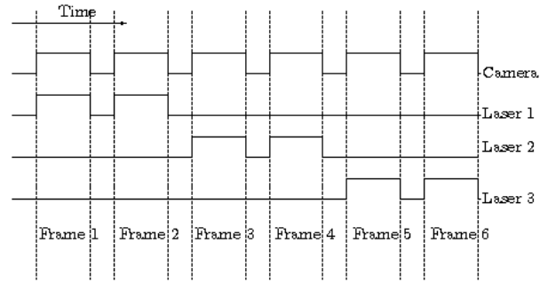
FIG. 2. Timing diagram over 6 frames showing the firing sequence of the camera and 3 lasers, the full 3D PIV system typically cycles over 10 lasers and 20 frames. While this shows 3 lasers the system has no limit in principle to the total number.
