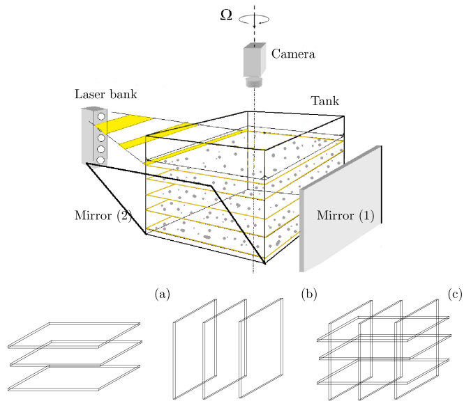
FIG. 1. Schematic diagram showing the experimental setup in the top panel and (a) 2D horizontal (b) 2D vertical and (c) 3D velocity grids. Mirror (1) is used to amplify the laser intensity and, as described in the text, Mirror (2) is used for 3D velocity extraction.
