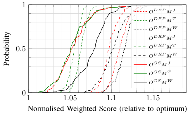
Figure 7: Cumulative Distribution Function graphs for heuristic algorithm outputs of schedule times and energy for Case 3 with w_t : 0.5 w_e : 0.5 (13 MDs, 3 MEC servers, 115 jobs).
