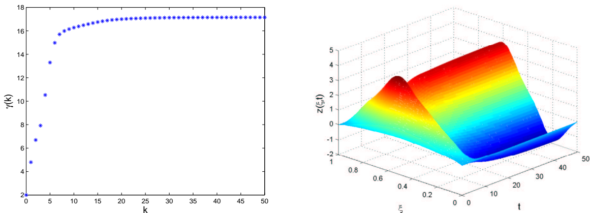
Figure 3.3: Sequence \gamma and temperature z(\xi, t) .
