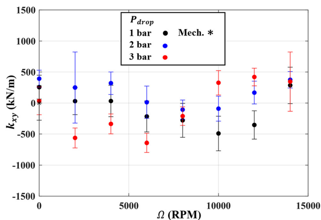
Fig. 15 Cross-coupled stiffness of the 4T brush seal with conventional back plate at different pressure drops and rotational speeds
