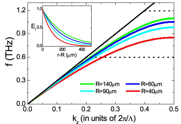
Fig. 6. Frequency versus parallel wavevector for spoof SPPs supported by metawires of different radii perforated with periodic ring arrays of period \Lambda = 100 \mu\text{m} and ring dimensions a = 50 \mu\text{m} and h = 30 \mu\text{m} . Dotted lines indicate two different frequencies (0.6 and 1.2 THz). Inset: Electric field radial component versus r - R at f = 0.6 THz for the four infinite metawires considered in the main panel.
