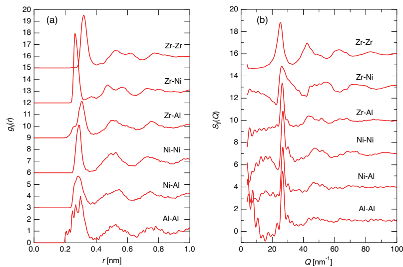
Figure 2. (Color online.) (a) g_{ij}(r) and (b) S_{ij}(Q) functions obtained from the RMC fits. For clarity, the spectra are displaced upwards by 3 each.
