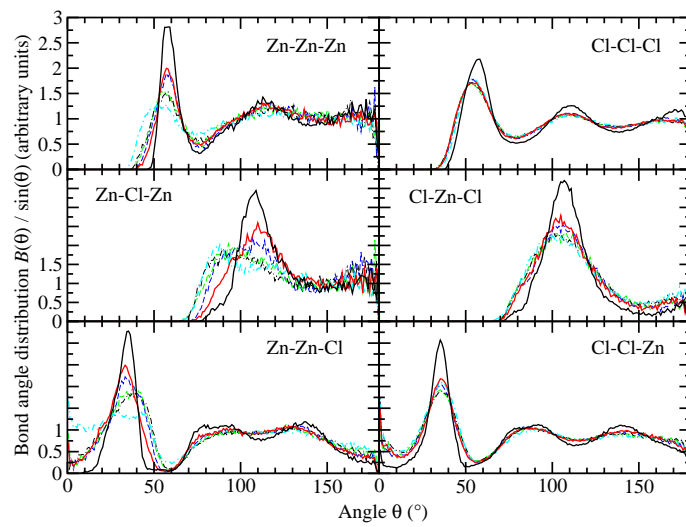
Figure 10: The bond angle distributions for the RMC models of glassy and liquid ZnCl 2 obtained in the present work. The identity of the curves is described in the Fig. 7 legend.
