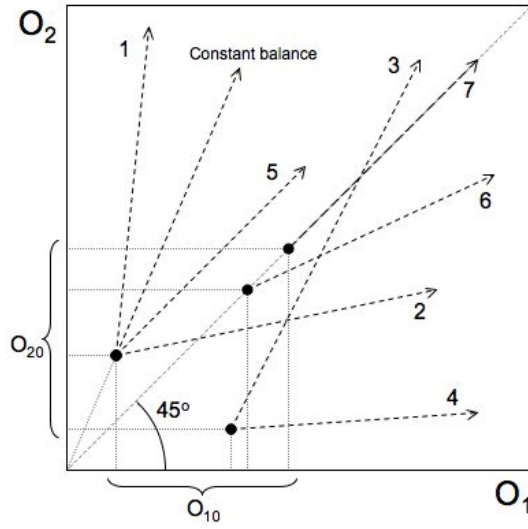
Figure 2: Trajectories of the two parent options in (O_1, O_2) space
