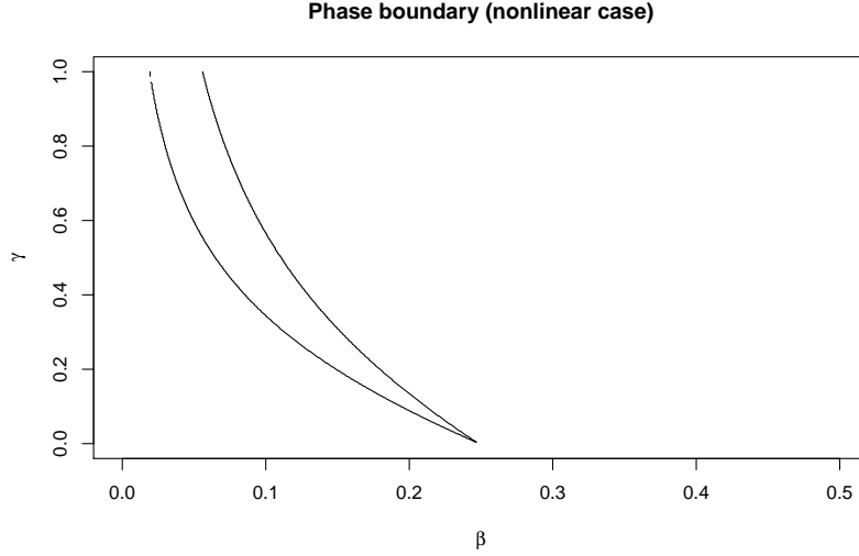
FIG 4. For the attachment function f(k) = \gamma\sqrt{k} + \beta the figure shows the curves a[f] = \frac{1}{2} and a[f] + \sqrt{a[f]c[f]} = 1 , which form lower and upper bound for the boundary between the two phases, nonexistence and existence of the giant component, in the (\beta, \gamma) -plane.
