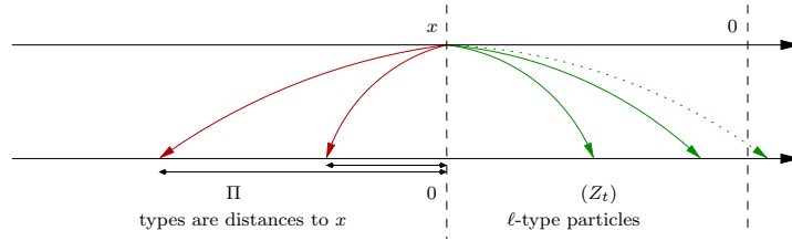
FIG 1. Offspring of an \ell -type particle in the branching random walk. A particle generates finitely many offspring to its left, but infinitely many offspring to its right.
