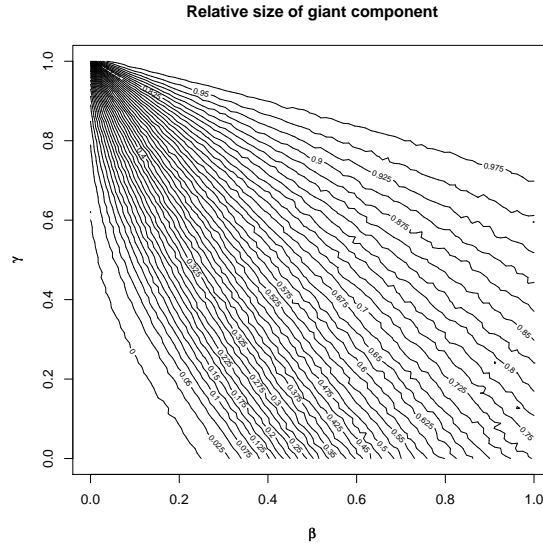
FIG 3. Simulation of the proportion of vertices in the giant component in the linear case. The curve forming the lower envelope is determined explicitly in Proposition 1.3. The plot is based on 15.000 Monte Carlo simulations of the branching process for 80 times 80 gridpoints in the (\beta, \gamma) -plane.
