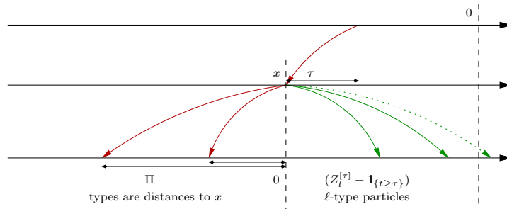
FIG 2. Offspring of a particle of type \tau \in [0, \infty) in the branching random walk. Offspring to the right have type \ell , offspring to the left have type given by the distance to the parent.
